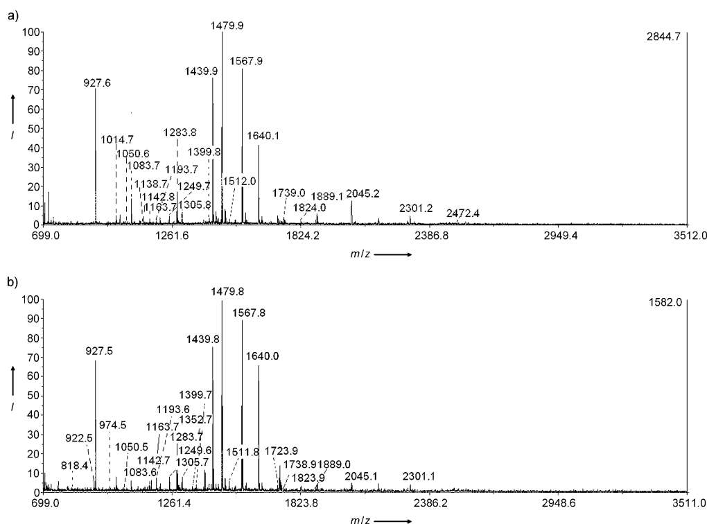
Figure 4. MALDI mass spectra of the extracted digests of 1 \mu\text{g} of BSA bands ( 1\ \mu\text{g}\ \mu\text{L}^{-1} \times 1\ \mu\text{L} ) from gel pieces obtained by a) laser-assisted in-gel digestion at 37°C for 45 s and b) conventional in-gel digestion at 37°C for 16 h. The peaks of all matched peptides are labeled with mass values.
