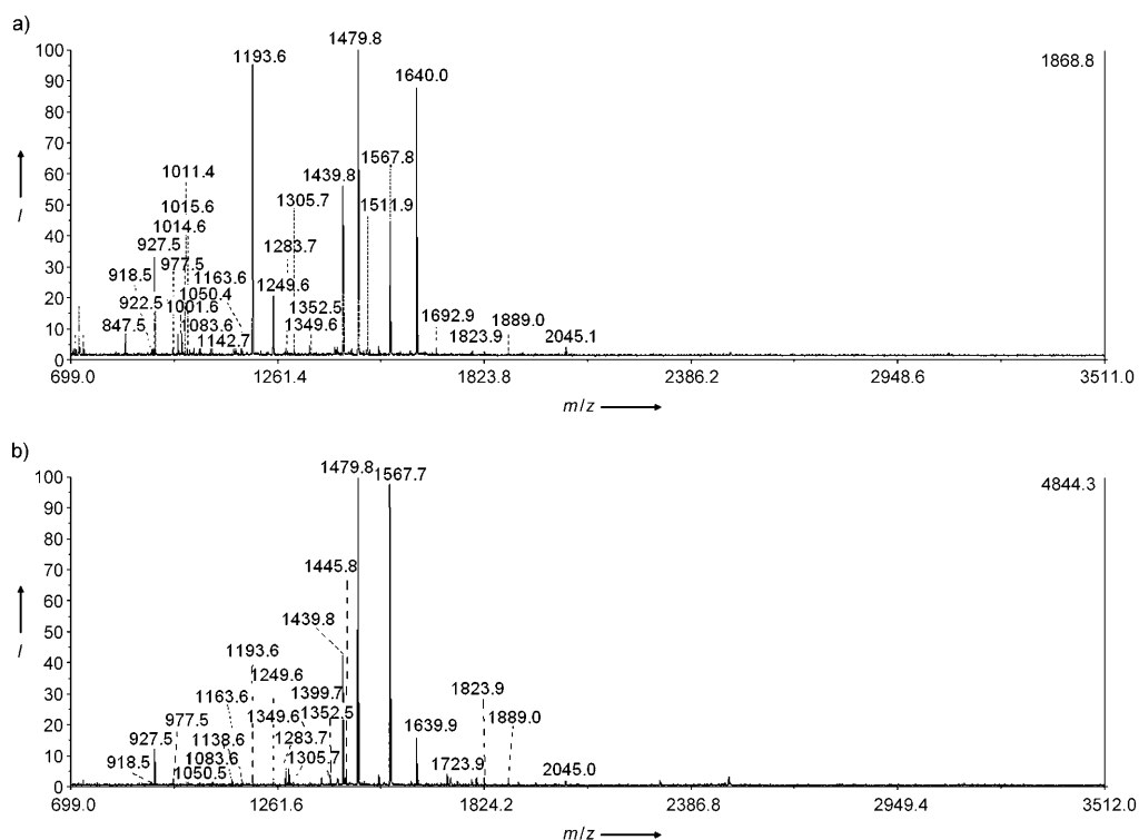
Figure 2. The MALDI mass spectra of digests of BSA obtained by a) laser-assisted in-solution digestion at 37°C for 45 s (power: 5W) and b) conventional in-solution digestion at 37°C for 12 h. The peaks of all matched peptides are labeled with mass values. Conditions: 1 \mu\text{L} trypsin ( 0.1 \mu\text{g} \mu\text{L}^{-1} )/20 \mu\text{L} proteins ( 0.2 \mu\text{g} \mu\text{L}^{-1} ). I = % intensity.
